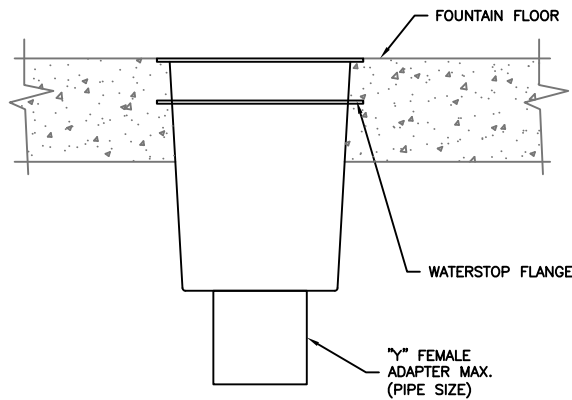
INSTALLATION DETAIL
