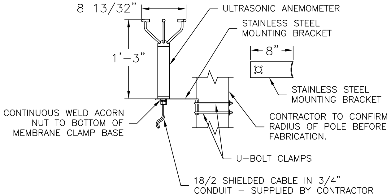
INSTALLATION DETAIL
